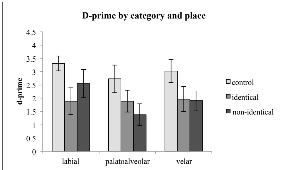
Figure 9: D-prime scores on control, identical and non-identical trials in the ABX experiment, by place of articulation. Error bars indicate Standard Error.
