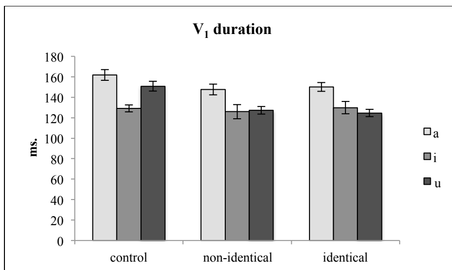
Figure 4: Duration of V 1 in correct productions of ejectives in the non-identical, identical and control categories, by vowel. Error bars indicate Standard Error. Control [a] n=58 , [i] n=37 , [u] n=82 ; non-identical [a] n=37 , [i] n=11 , [u] n=69 ; identical [a] n=60 , [i] n=24 , [u] n=82 .
