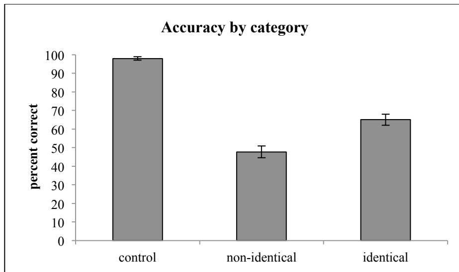
Figure 2: Accuracy on target items with medial ejectives in the phonotactically legal control category and the phonotactically illegal identical and non-identical categories. Error bars indicate standard error. Control category n=250 , non-identical n=245 , identical n=252 .
