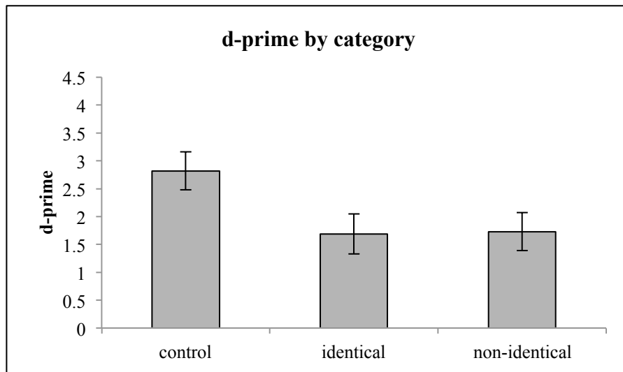
Figure 8: D-prime scores on control, identical and non-identical trials in the ABX experiment. Error bars indicate Standard Error.
