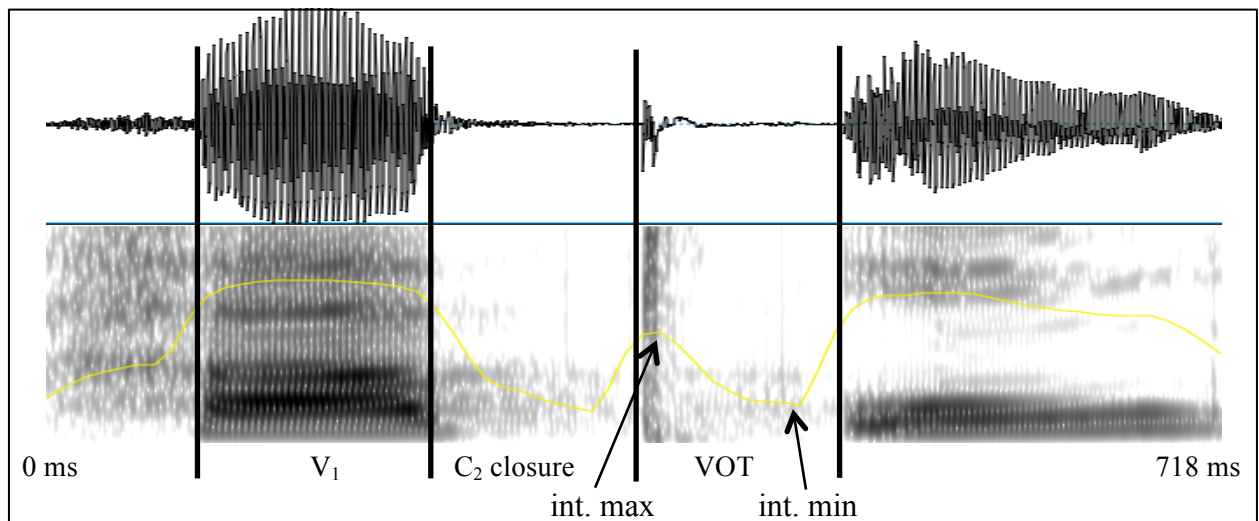
Figure 1: Spectrogram and waveform of [hap'u], showing landmarks for duration of V 1 , C 2 closure and VOT, and burst intensity measurements. Intensity window is 40-100 dB.
