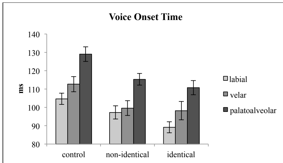
Figure 6: Duration of VOT in correct productions of ejectives in the non-identical, identical and control categories, by place of articulation. Error bars indicate Standard Error. Control labial n=79 , palatoalveolar n=75 , velar n=77 ; non-identical labial n=40 , palatoalveolar n=29 , velar n=46 ; identical labial n=50 , palatoalveolar n=49 , velar n=62 .
