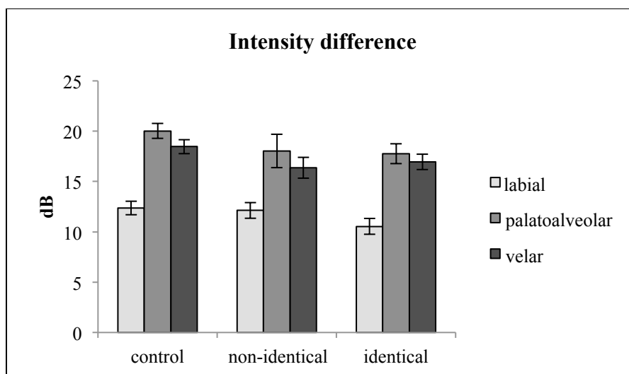
Figure 7: Intensity difference during burst and VOT period in correct productions of ejectives in the non-identical, identical and control categories, by place of articulation. Error bars indicate Standard Error. Control labial n=79 , palatoalveolar n=75 , velar n=77 ; non-identical labial n=40 , palatoalveolar n=29 , velar n=46 ; identical labial n=50 , palatoalveolar n=49 , velar n=62 .
