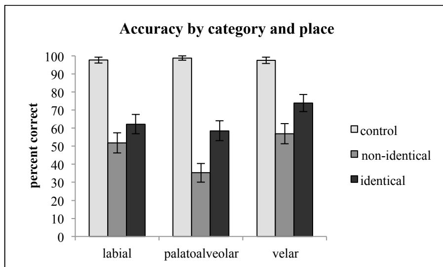
Figure 3: Accuracy on target items with medial ejectives, by category and place of articulation. Error bars indicate standard error. Labials: control n=86 , non-identical n=81 , identical n=82 , palatoalveolars: control n=84 , non-identical n=85 , identical n=82 , velars: control n=80 , non-identical n=79 , identical n=88 .
